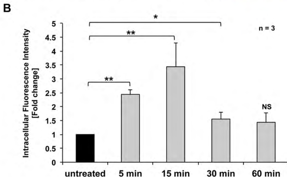
FIGURE 1: VEGF induces rapid, transient Cx43-GJ internalization in PAECs. (A) Double staining of Cx43 (green) and ZO-1 (red) in untreated cells (a–c), or in cells treated with 100 ng/ml VEGF for 5 (d–f), 15 (g–i), 30 (j–l), or 60 (m–o) min. Nuclei were stained with Hoechst 33342 (blue). Representative images acquired with identical camera settings are shown. Note the acute transient loss of plasma membrane-localized GJs and a simultaneous increase in punctate, intracellular Cx43 fluorescence. (B) Normalized quantitative analyses of intracellular fluorescence intensity of Cx43 (an indirect measure of reduced plasma membrane fluorescence intensity) in untreated and VEGF-treated cells at indicated time points of three independent experiments (a total of >300 cells). Significant differences are depicted with asterisks.
