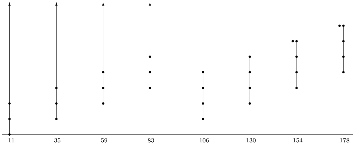
Diagram 3.6. UASS(B(11, 35, 59, 83)_{13}) in dim < 200 .
