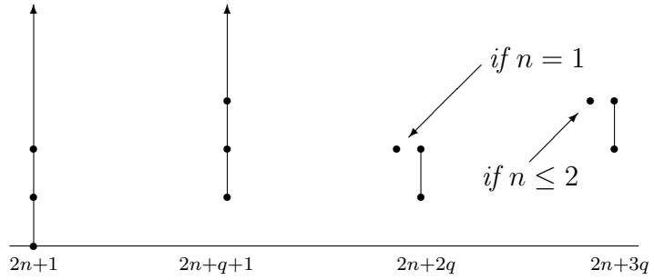
Diagram 3.6. UASS(B(11, 35, 59, 83)_{13}) in dim < 200 .
