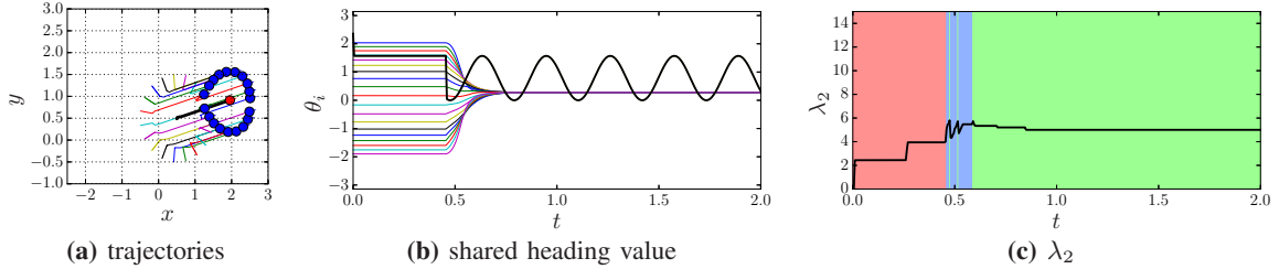
Fig. 5: Simulation results using the proposed controller in which a non-cooperative robot shares a time-varying signal with its neighbors. The bold black line in (b) shows the shared value of the non-cooperative robot. In (c) the vulnerable, marginal, and resilient states are shown in red, blue, and green.
