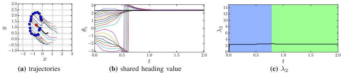
Fig. 7: Simulation results when robots maintain \lambda_2 > 2 instead of the resilience threshold in the presence of one non-cooperative robot. The bold black line in (b) shows the shared value of the non-cooperative robot.
