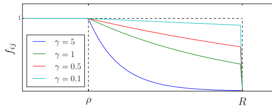
Fig. 1: The effect of design parameter \gamma on communication function f_{ij} . The x-axis is the distance between agents, \|\mathbf{x}_i - \mathbf{x}_j\| .
