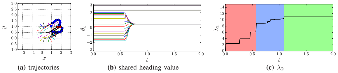
Fig. 4: Simulation results using the proposed controller with two non-cooperative robots. The non-cooperative robots are shown in red in (a) and in (b) the bold black lines show the values they are sharing with their neighbors. In (c) the vulnerable, marginal, and resilient states are shown in red, blue, and green.
