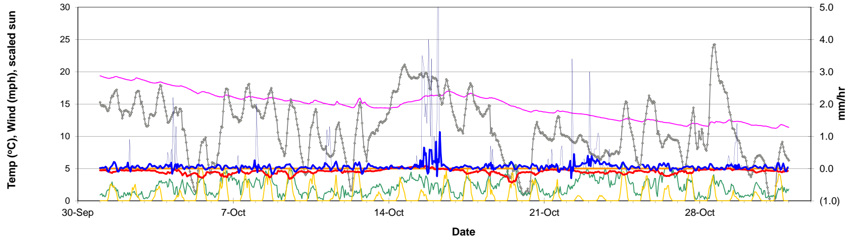
L. Lacawac Wthr & calc hourly data: Lake Evap_chg, Residual_chg; Resid. lakechg >0 = runff (incl snowmelt) into lake or snow on lake, <0 is gage melt
