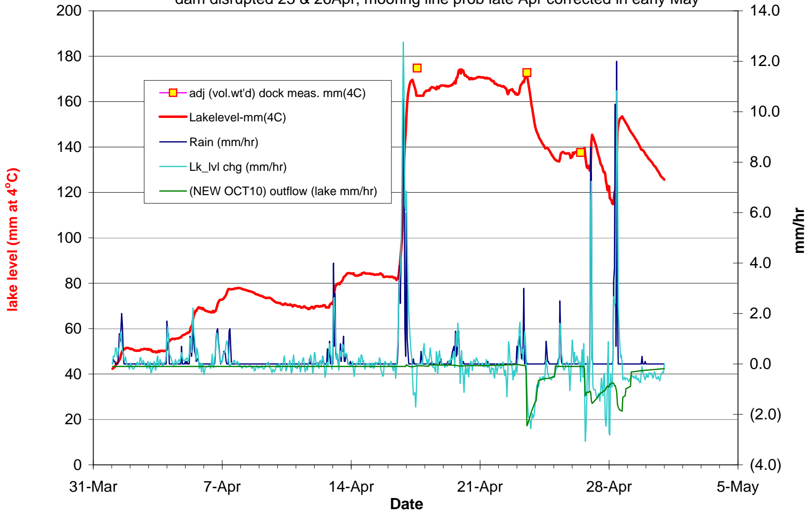
L. Lacawac Hourly avg Lake level, Lake level change/hr, Rain/hr Snow: 1Apr=1"; beavers back in April (stream outflow model requires high sill to match lake level chgs); dam disrupted 23 & 26Apr; mooring line prob late Apr corrected in early May
