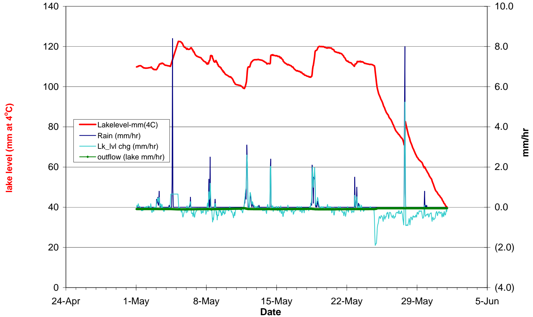
L. Lacawac Hourly avg Lake level, Lake level change/hr, Rain/hr Beaver dam established late April partly disrupted 21, 24May; stream flow not adjusted yet for logged in-stream level
