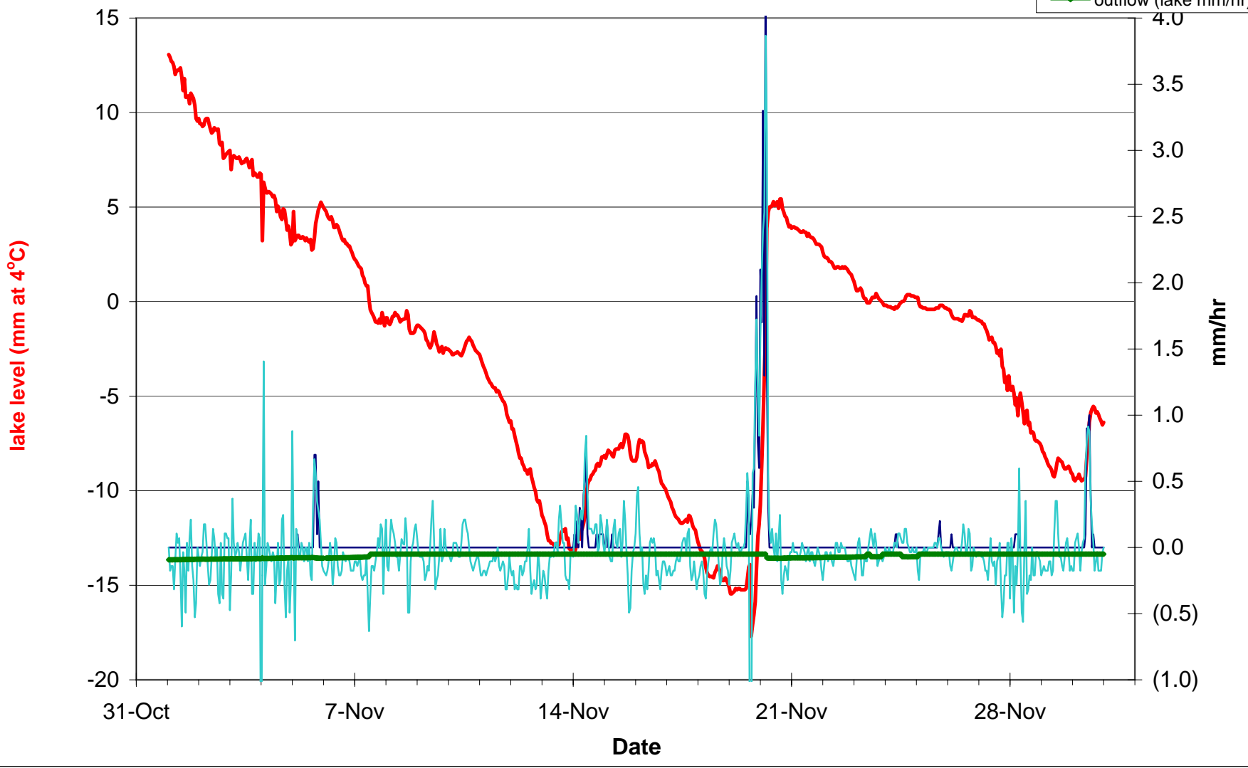
L. Lacawac Hourly avg Lake level, Lake level change/hr, Rain/hr Increased lakelevel noise starting 19Oct (anchor line problem?); platform moved to dock 8Nov another shift on 11/19?
