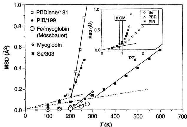
Fig. 11. Variations of the Debye-Waller factor, \langle r^2 \rangle with T_g -scaled temperature, showing change of slope around the temperature of the calorimetric glass transition, T_g . T_g values in Kelvin degrees are given in legend; PBDiene, polybutadiene, and PIB, polyisobutylene. Insert shows the same data versus T/T_g , except for proteins for which T_g is only ambiguously defined by calorimetry. The band marked 8 OM shows the reduced temperature range needed to change the relaxation time of a fragile liquid, o-terphenyl, by eight orders of magnitude.
