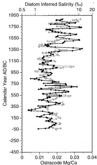
FIG. 5. Comparison of Coldwater Lake diatom-inferred salinity (black) and ostracode Mg/Ca (gray).
