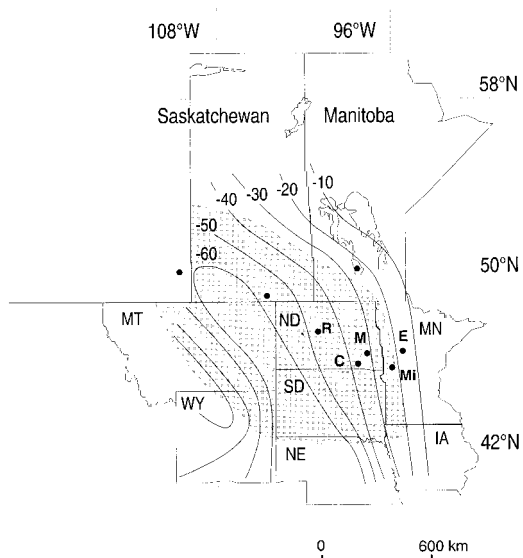
FIG. 1. Map of the northern Great Plains (shaded area) showing the location of Moon (M), Coldwater (C), Rice (R), Elk (E), and Mina (Mi) lakes. Isolines are of precipitation minus evaporation (in cm). Figure modified from Winter and Woo (1990).
