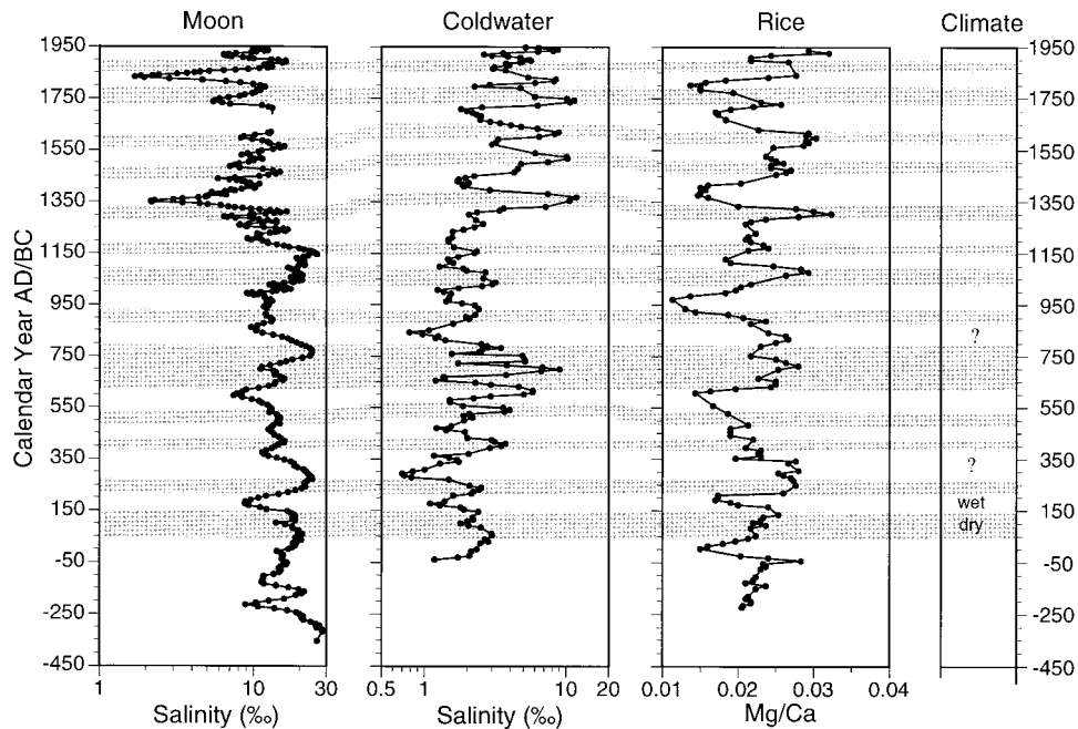
FIG. 2. Diagram showing patterns of salinity change at the three lake sites in the northern Great Plains, arranged east (Moon) to west (Rice). Data from Coldwater and Rice lakes are smoothed with a 3-point running average and from Moon Lake with a 6-point running average. The gap in the Moon Lake record around A.D. 1600 is the result of desiccation of the core; thus, data are unavailable for this period. Shaded intervals represent times of major drought. Unshaded intervals indicate wetter periods, except for intervals where the three records differ, which are marked with question marks.
