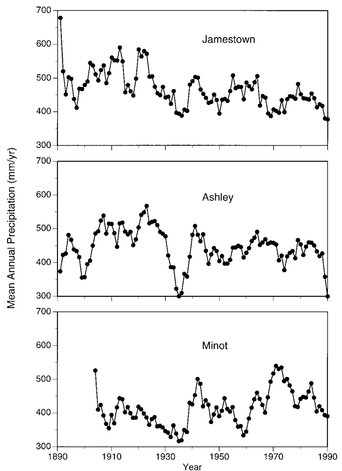
FIG. 6. Mean annual precipitation ( \text{mm yr}^{-1} ) in the 20th century for the three climate stations closest to the three North Dakota lake sites discussed in the text. Data are smoothed with a 5-point running average.
