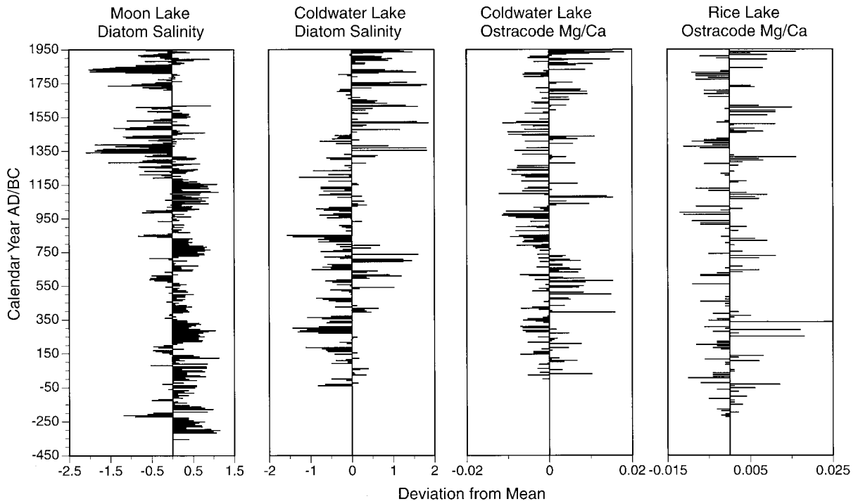
FIG. 3. Deviation from the 2000-yr lake-water chemistry mean for the proxy records from Moon, Coldwater, and Rice lakes.
