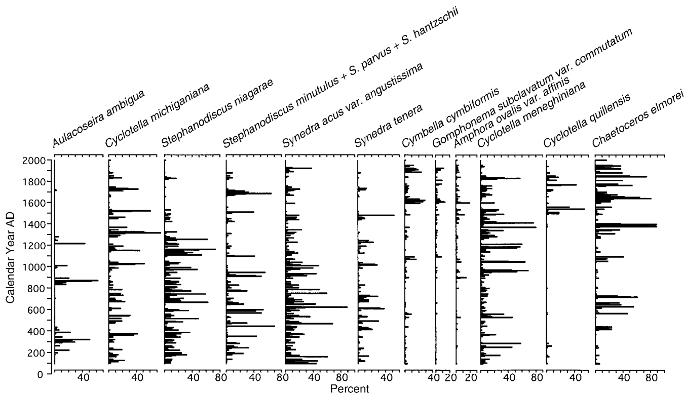
FIG. 4. Summary diatom diagram of the major taxa used to infer salinity variations in Coldwater Lake.
