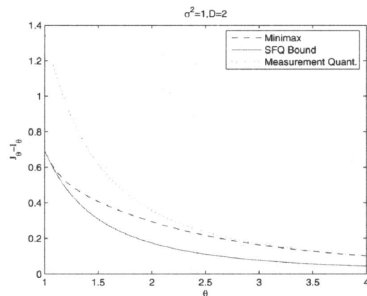
Fig. 5. Minimax Quantizer
