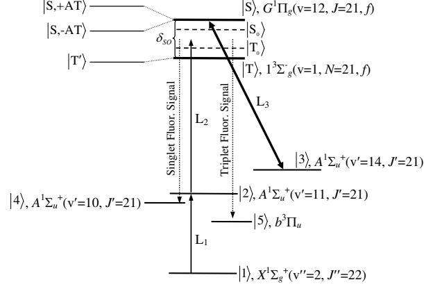
FIG. 1: Thermal population in level |1\rangle is excited to level |2\rangle by the weak pump laser L_1 ( 15810.158 \text{ cm}^{-1} ), and then further excited by tuning the weak probe field L_2 to the mixed pair of levels |T\rangle and |S\rangle , with resonances at 17666.136 \text{ cm}^{-1} and 17666.162 \text{ cm}^{-1} , respectively. Laser L_3 is set on resonance with the |S\rangle \leftrightarrow |3\rangle transition at 17026.872 \text{ cm}^{-1} . Levels |S_0\rangle and |T_0\rangle are the 'pure' singlet and triplet basis states, respectively (unperturbed basis set). With the control laser on, |S\rangle and |T\rangle evolve into |S, -AT\rangle , |S, +AT\rangle , and |T'\rangle . The parameters \mu_1 = 2.1 \text{ D} , \mu_2 = 1.8 \text{ D} , \mu_3 = 3.3 \text{ D} , \tau_2=18.78 \text{ ns} , \tau_{S_0}=16.21 \text{ ns} , \tau_{T_0}=9.27 \text{ ns} , and \tau_3=18.90 \text{ ns} were calculated from molecular data [20, 22–25] using LEVEL [26].
