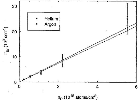
FIG. 6. Plot of \Gamma_{\text{br}} vs n_p (for Ar and He perturber atoms) for the 553.5-nm ^1S_0 \rightarrow ^1P_1 barium resonance transition. k_{\text{br}} values are determined from the slopes of the solid (He) and dashed (Ar) least-squares-fitted lines.
