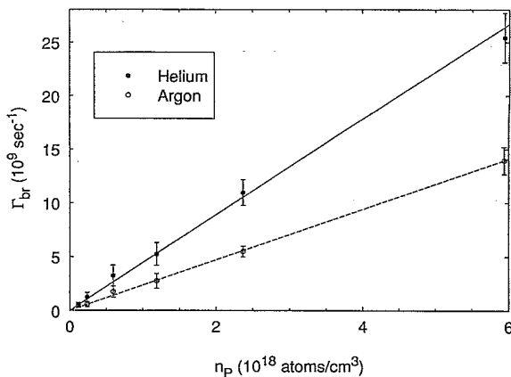
FIG. 4. Plot of \Gamma_{br} vs perturber density n_p for the 791.1-nm ^1S_0 \rightarrow ^3P_1 intercombination line using both He and Ar perturber atoms. The solid and dashed lines are the least-squares fits for He and Ar buffer gas, respectively. k_{br} is determined from the slopes of these lines.
