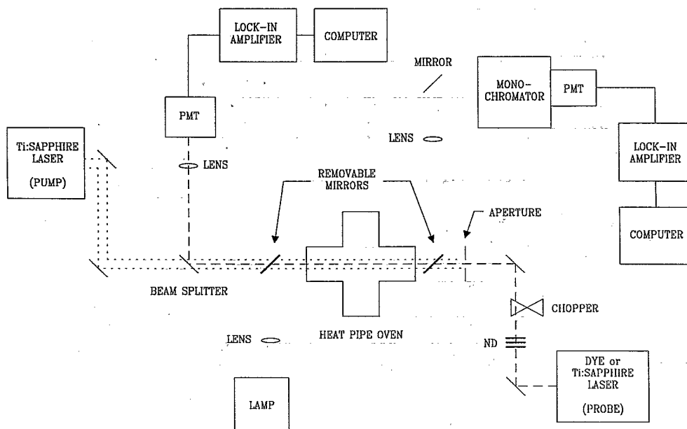
FIG. 2. Experimental setup used for the three types of measurements reported in this work. For measuring broadening and shift rates of the intercombination line at 791.1 nm, only the highly attenuated Ti:sapphire probe laser was used. For studies of the ^3D_2 level, the full power ( \sim 200 mW) of the Ti:sapphire pump laser was used as the pump, while the highly attenuated dye laser was used as the probe. Finally, for investigations of the resonance transition, the removable mirrors were inserted into the setup and frequency-dependent transmission of the white light was monitored using the monochromator-PMT with all lasers off. PMT and ND represent photomultiplier tube and neutral density filter, respectively.
