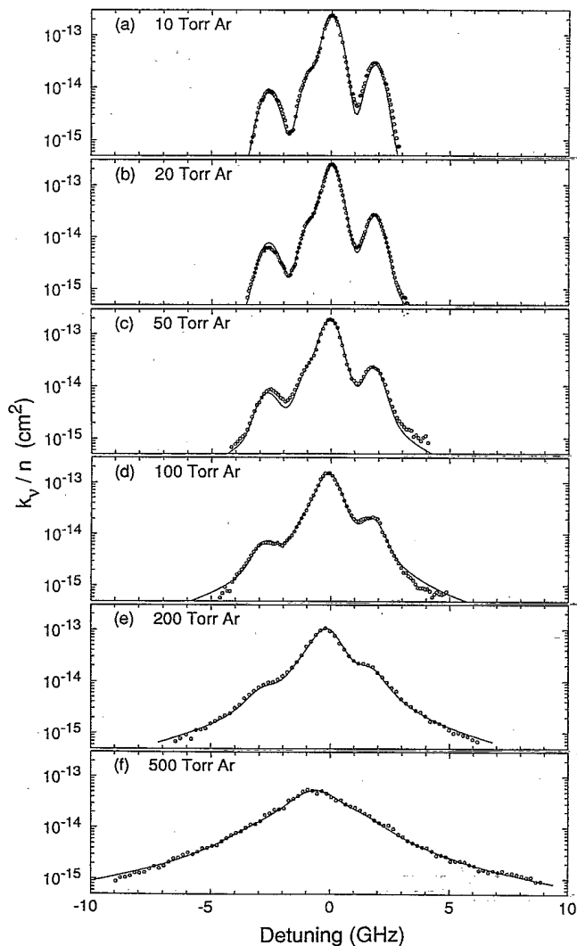
FIG. 3. Comparison of the experimental 6s^2^1S_0 \rightarrow 6s6p^3P_1 transition line shapes (data points) at various Ar pressures with the composite Voigt line shapes that were calculated using the measured value of k_{br}^{\text{Ar}} (solid lines).
