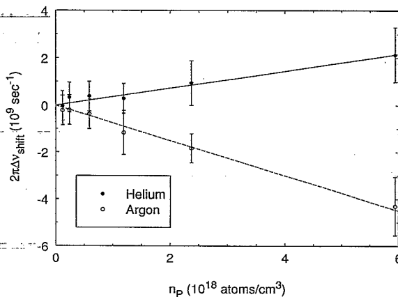
FIG. 5. Plot of collisional line shifts vs n_p for the 791.1-nm ^1S_0 \rightarrow ^3P_1 intercombination line using both He and Ar perturbors. The solid and dashed lines are the least-squares fits for He and Ar buffer gas, respectively. Slopes of these lines yield k_{\text{shift}} .
