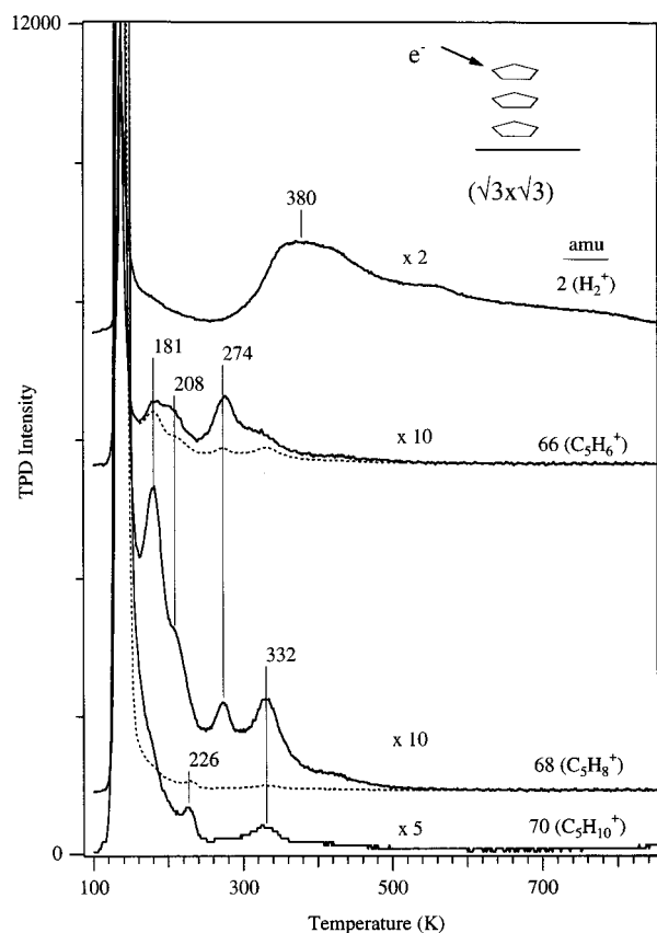
Figure 4. TPD spectra after EID of a 3-ML cyclopentane ( c\text{-C}_5\text{H}_{10} ) film on the \sqrt{3} alloy at 100 K.
