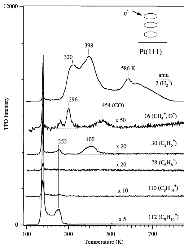
Figure 9. TPD spectra after EID of a 3-ML cyclooctane ( c\text{-C}_8\text{H}_{16} ) film on Pt(111) at 100 K.
