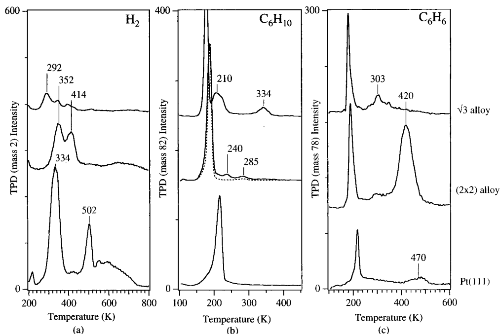
Figure 13. Comparison of TPD spectra after EID of cyclohexane (c-C 6 H 12 ) films on Pt(111) and Pt-Sn surface alloys at 100 K: (a) hydrogen (H 2 ); (b) cyclohexene (c-C 6 H 10 ); (c) benzene (C 6 H 6 ).
