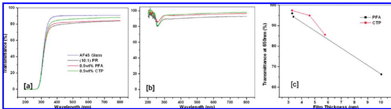
FIGURE 4. Comparison of the transmittance of carbon-coated glasses as measured using UV–vis spectroscopy with respect to (a) air as the reference and (b) the bare glass substrate as the reference. (c) Change in the transmittance as a function of the film thickness of the carbon layer on AF45 glass.
