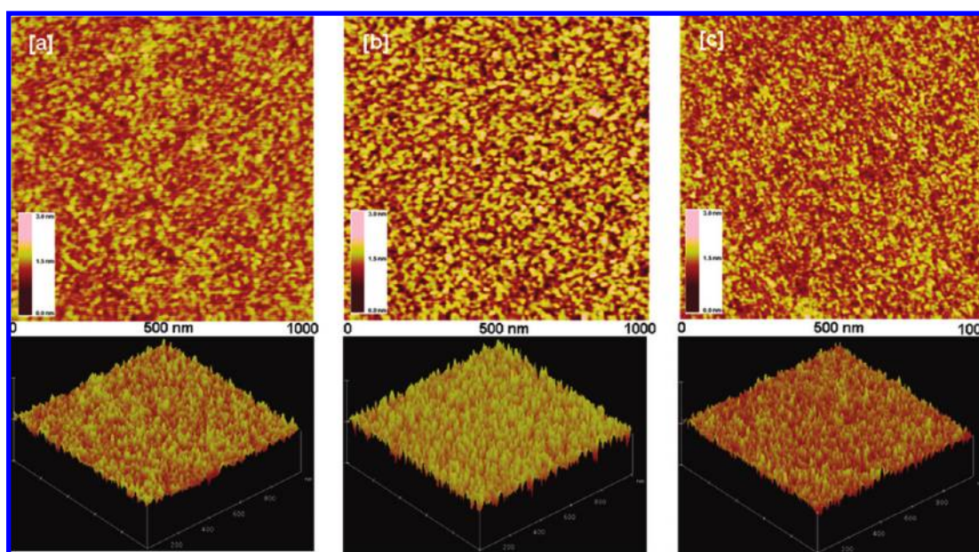
FIGURE 2. AFM topographical images (flattened images and 3D images) ( 1 \mu\text{m} \times 1 \mu\text{m} ) of the deposited carbon layer: (a) 1 wt % PFA, rms roughness = 0.190 \pm 0.027 \text{ nm} ; (b) 5 wt % CTP, rms roughness = 0.293 \pm 0.036 \text{ nm} ; (c) PR (10:1), rms roughness = 0.180 \pm 0.021 \text{ nm} .
