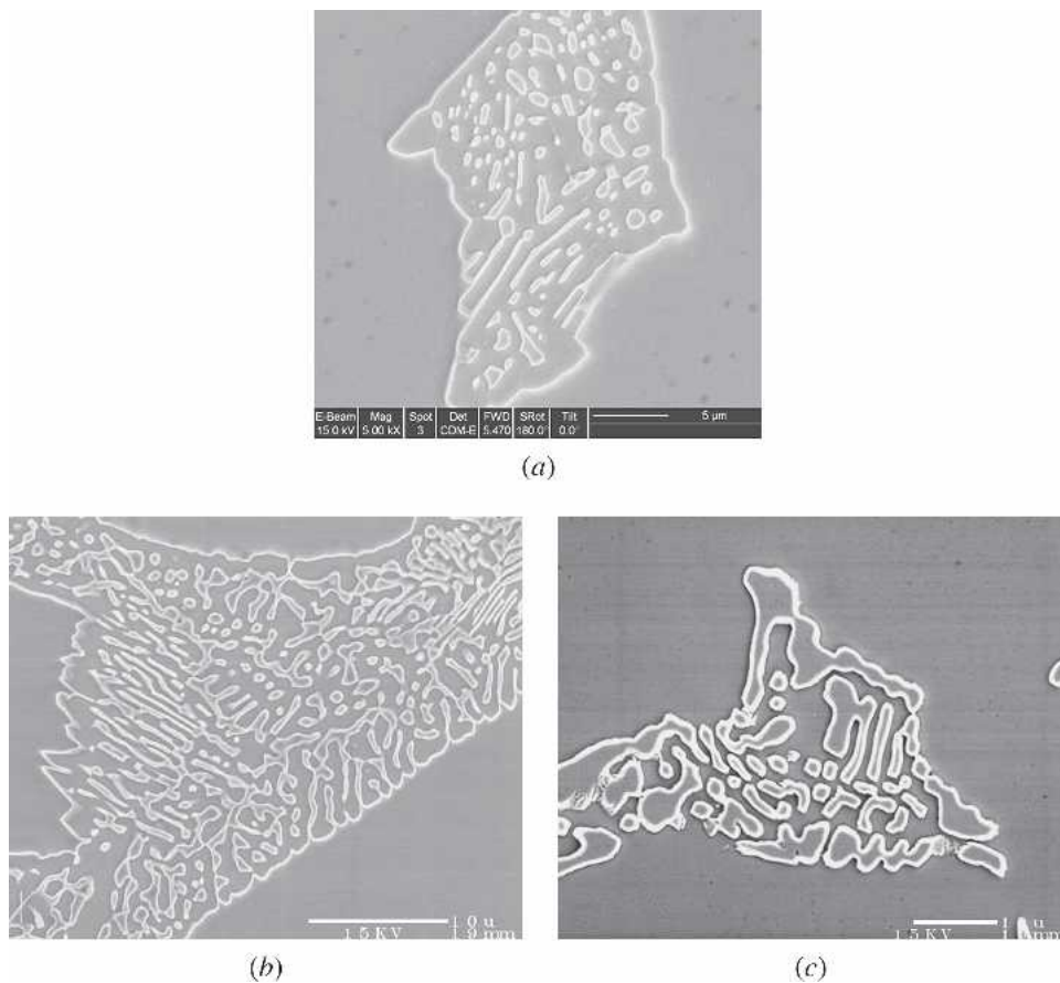
Fig. 4—Comparison of eutectic morphologies observed in a scanning electron microscope for DTA specimens: (a) AL-6XN exhibits eutectic with an intermetallic and \gamma -austenite islands, (b) Fe-base alloy 1 exhibits similar eutectic morphology to AL-6XN but with regions of lamellar structure, and (c) Ni-base alloy 3 showing a eutectic morphology with large blocky islands of intermetallic in the \gamma matrix. All samples are electrolytically etched with 60 pct \text{HNO}_3/40 pct \text{H}_2\text{O} mixture.
