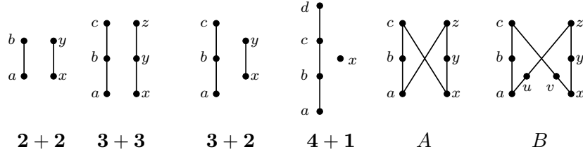
Figure 4: Orders that appear as separating examples in Figure 3.
