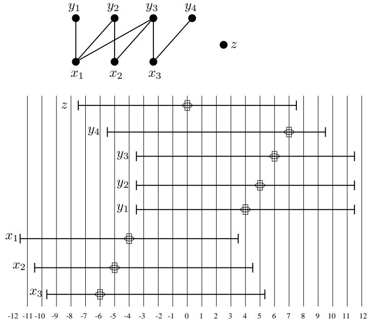
Figure 8: An ordered set and a unit point-core bitolerance representation of it.
