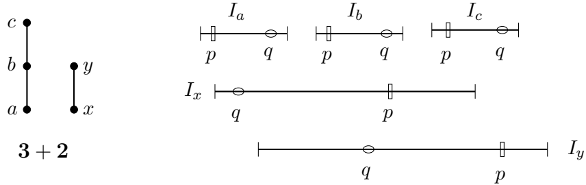
Figure 1: The order \mathbf{3 + 2} and a bounded bitolerance representation of it.
