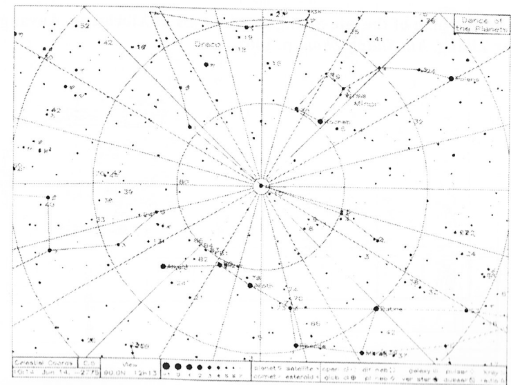
Fig. 7: Thuban, the late-Neolithic pole-star, at 90° N in 2,775 BCE ( Dance of the Planets © ARC Software).
