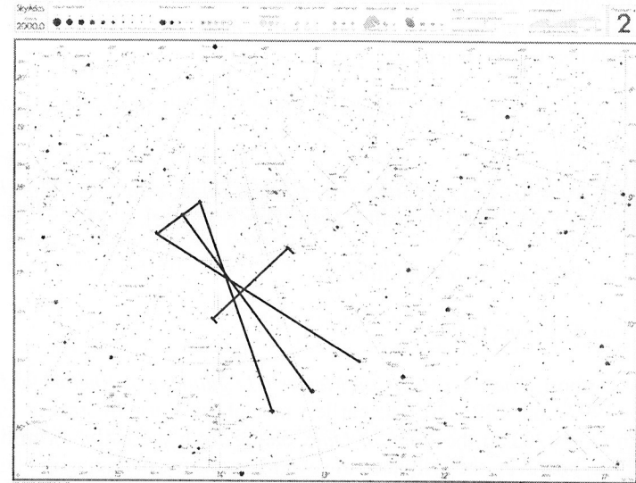
Fig. 13: Star chart showing the location of the north celestial pole in 2,000 BCE ( Dance of the Planets © ARC Software).
