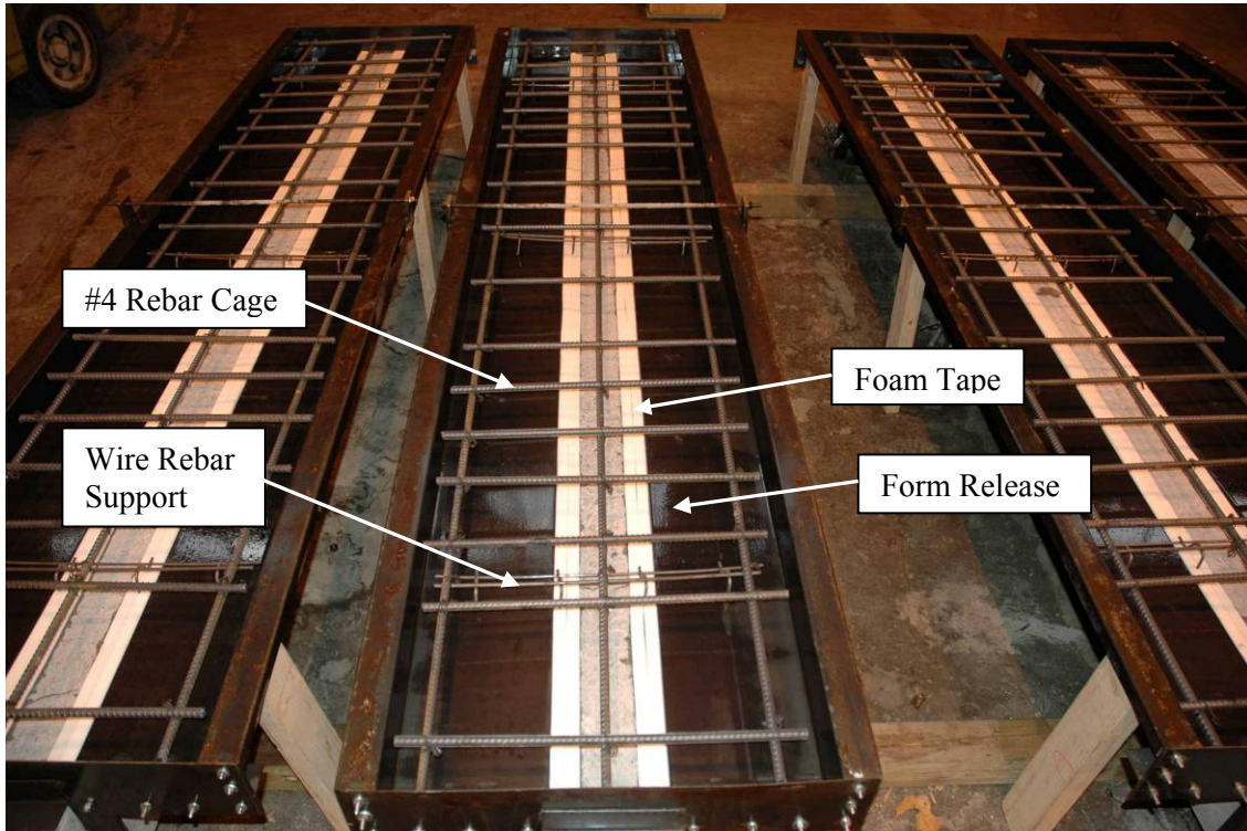
Figure 7-22: Pour-Ready Setup
