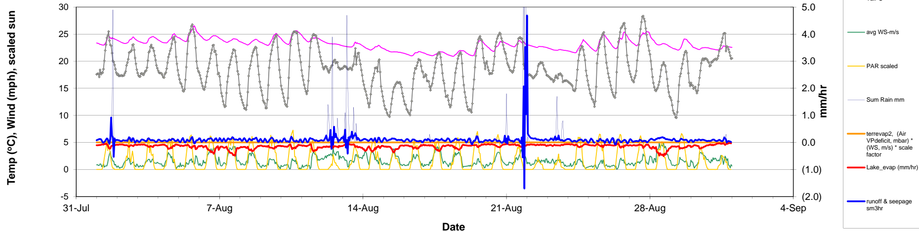
L. Lacawac Wthr & calc hourly data: Lake Evap_chg, Residual_chg); Resid. lakechg >0 = runff (incl snowmelt) into lake or snow on lake, <0 is gage melt
