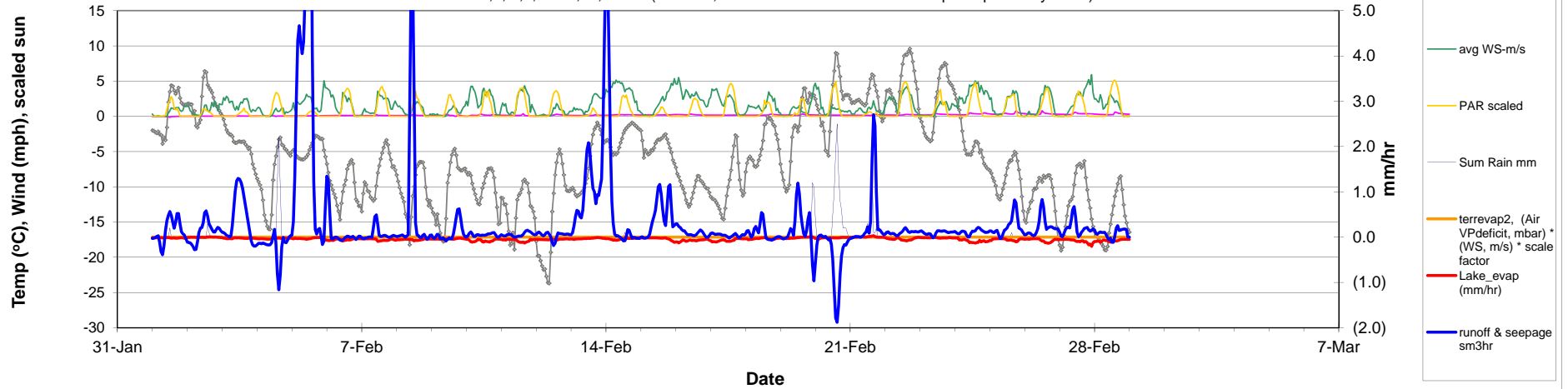
L. Lacawac Wthr & calc hourly data: Lake Evap_chg, Residual_chg); Resid. lakechg >0 = runff (incl snowmelt) into lake or snow on lake, <0 is gage melt; NWS: NWS snow 3,5,8 ,9,13-16,18,19Feb (on 5Feb, much more than 26mm water equiv reported by NWS) Feb
