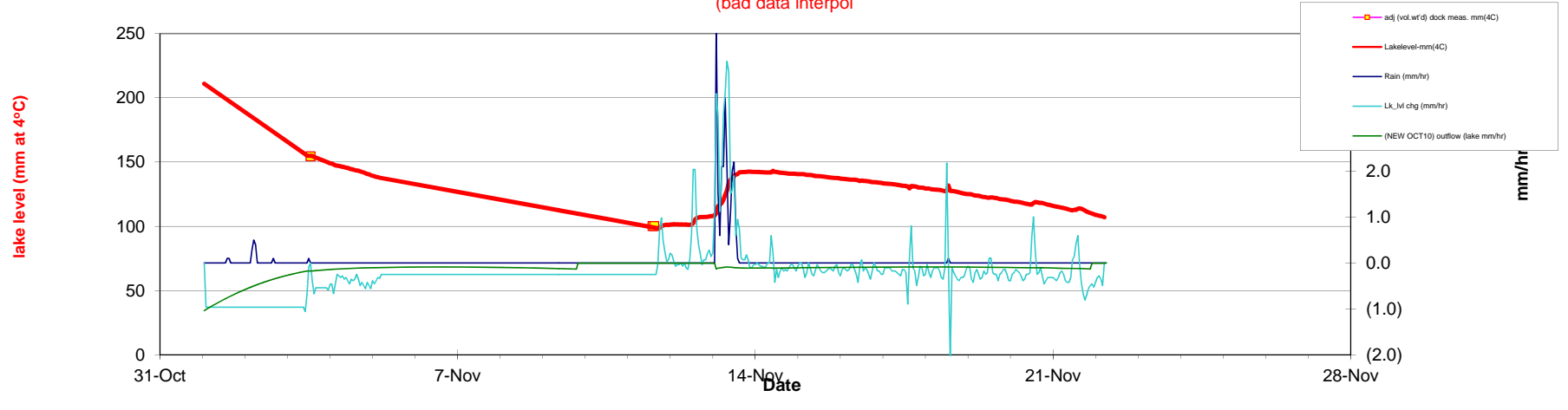
L. Lacawac Hourly avg Lake level, Lake level change/hr, Rain/hr TO LAKE CENTER 24MAR2012 May: Beavers are back; adjustments to drain on 13June. Lake level sensor vent tube broken and sensor dragged by "Sandy" 29Oct2012; replaced 11Nov12 (bad data interpol)
