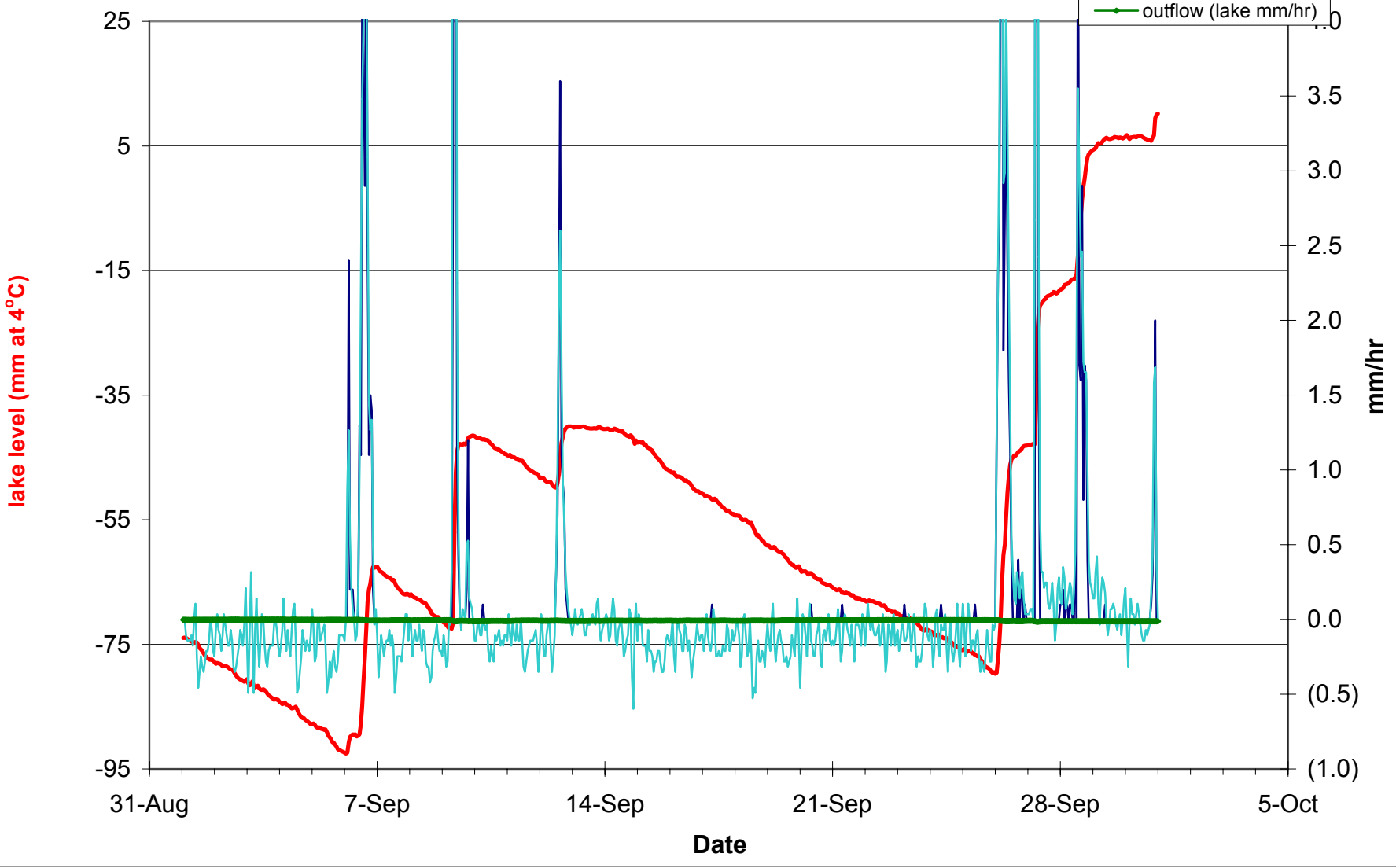
Hourly avg Lake level, Lake level change/hr, Rain/hr beaver dams observed 16Apr08; partly disrupted 5 & 22 Jun, 4Jul 08
