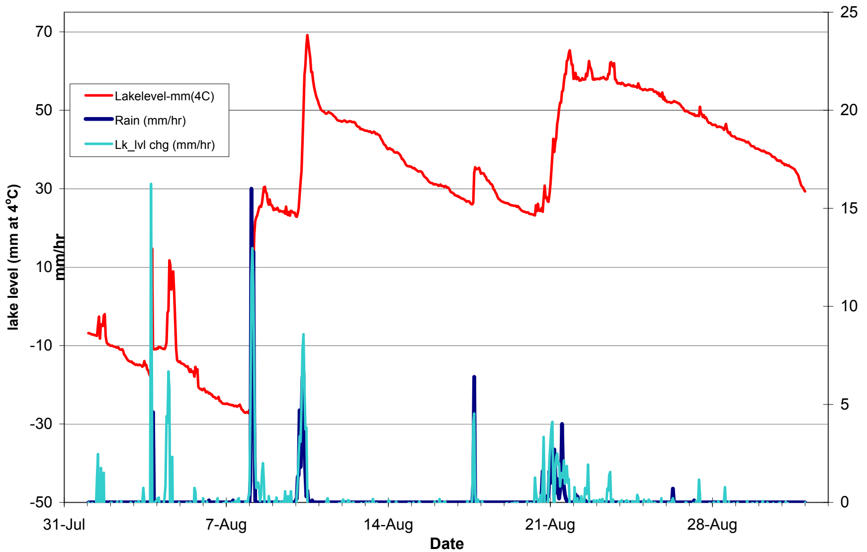
Hourly avg Lake level, Lake level change/hr, Rain/hr (spikes in lake level caused by water in sensor air vent?)
