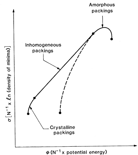
Fig. 4. Logarithm of the distribution of potential energy minima, plotted against potential energy per particle. The case shown corresponds to a pure substance that has a first-order melting transition.
