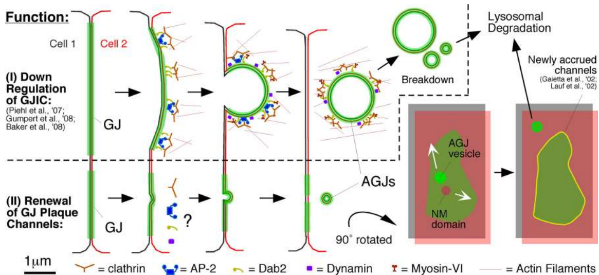
Figure 7. Schematic representation of the pathways that lead to GJ plaque internalization (described in Piehl et al. , 2007; Baker et al. , 2008; Gumpert et al. , 2008) (I) and GJ plaque channel renewal (described here), GJ vesicle formation (AGJ), and GJ vesicle degradation (II). Whether clathrin and clathrin accessory proteins are involved in the internalization of small GJ vesicles described here has not been determined; however, is probably based on our electron microscopy analyses (see Figure 3). Displacement of nonjunctional membrane domains from central plaque areas (NM domain, gray/red) by lateral movement allows the simultaneous accretion of new channels (yellow) along the periphery of GJ plaques (green) without increasing plaque size consistent with previously published observations (Gaietta et al. , 2002; Lauf et al. , 2002). Clathrin and accessory proteins are shown in patches in accordance to the appearance of clathrin on GJ plaques (Piehl et al. , 2007), and the current thinking that clathrin may provide a scaffold for directed actin assembly, facilitating internalization of large structures such as GJs, viruses, and pathogenic bacteria (Pauly and Drubin, 2007; Veiga et al. , 2007). The manner in which clathrin and accessory proteins are drawn remains speculative.
