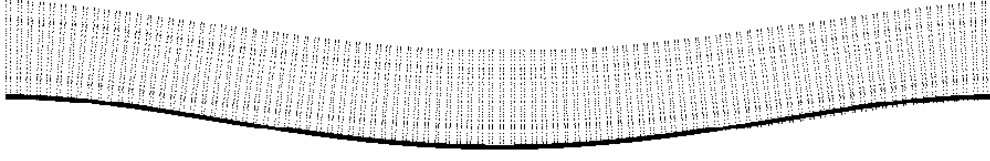
Figure 4. Comparison of the deflection of a 20 nm long fixed–fixed DWNT (diameter of 1.96 nm) with the deflection predicted by the beam equation. The solid black curve is the deflection predicted by the beam equation.
