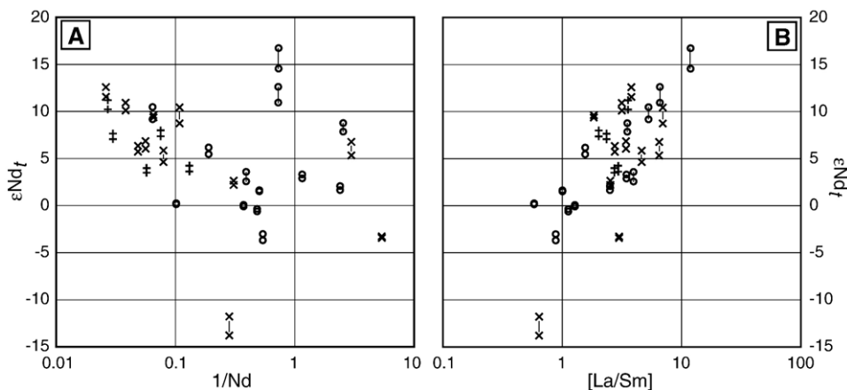
Fig. 9. Nd isotope-element mixing diagrams. Tie lines are shown connecting the two age corrections used for each sample; tie lines are not shown for samples where the two symbols overlap. See text for details regarding age correction of isotope ratios. Nd data suggest a binary mixing array between a positive \epsilon\text{Nd} , high Nd concentration, LREE-enriched source with a negative \epsilon\text{Nd} , low Nd concentration, LREE-depleted composition. The mixing array is probably controlled by mechanical mixing as little evidence for modification of this array by fluid flow is evident, in contrast to our interpretation of Sr isotope systematics.
