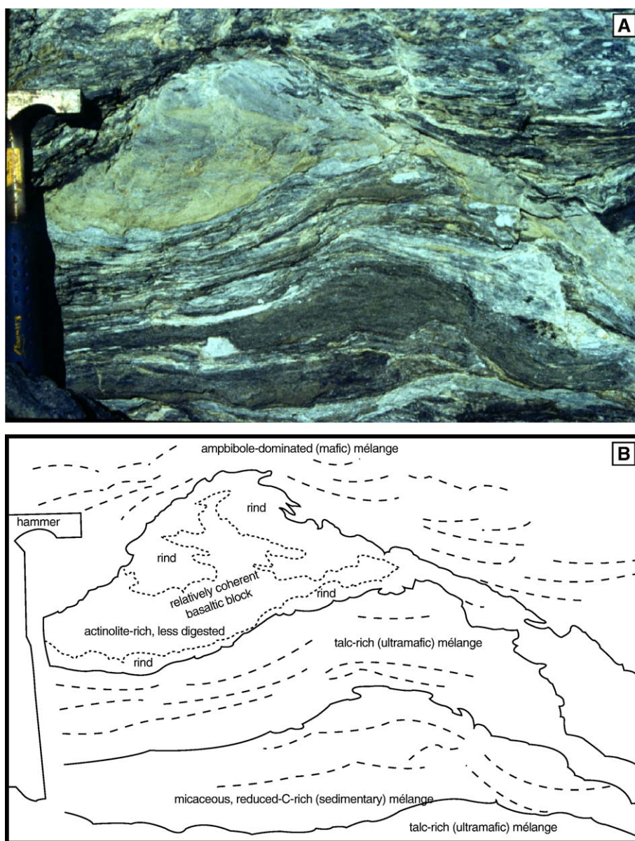
Fig. 1. Representative field photograph (A, above) and interpretative sketch (B, below) of meso-scale metamorphic and deformational features in lawsonite–albite facies mélange matrix of the Catalina Schist, CA. Solid lines denote contacts, dashed lines represent foliation. At left center is a large metabasaltic block bearing metasomatic rinds (dotted lines demarcate rind zones) within highly foliated mélange matrix. This exposure preserves amphibole-dominated ( \sim mafic) mélange matrix, talc-dominated ( \sim ultramafic) mélange matrix, and micaceous, reduced C-rich ( \sim sedimentary) mélange matrix. Note that the coherent block records progressive disaggregation via boudinage, focused along rind/ mélange contacts.
