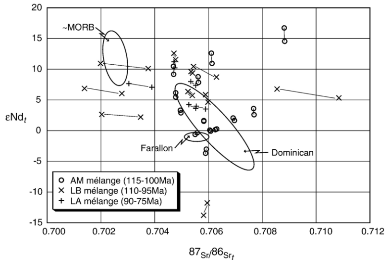
Fig. 7. Sr–Nd isotope data for mélangé matrix of the Catalina Schist presented as initial isotope ratios. Isotope compositions are age corrected for a range in ages due to uncertainty in the precise age of the mélangé matrix; age ranges based on Ar–Ar closure ages of [18]. Lines connect age corrections of individual samples; symbols and ages for correction given in the legend. Errors based upon age corrections greatly exceed all analytical errors. Oval labeled “MORB” represents an approximate Sr–Nd composition for mid-ocean ridge basalts. Oval labeled “Farallon” indicates the range in Sr–Nd composition for omphacite mineral separates from lawsonite eclogite xenoliths from the Colorado Plateau demonstrated to have originated as fragments of the subducted Farallon plate and of approximate MORB parentage [41,42]. Oval labeled “Dominican” is for the Sr–Nd compositions of metabasaltic blueschists and eclogites of the Dominican Republic as reported by [40].
