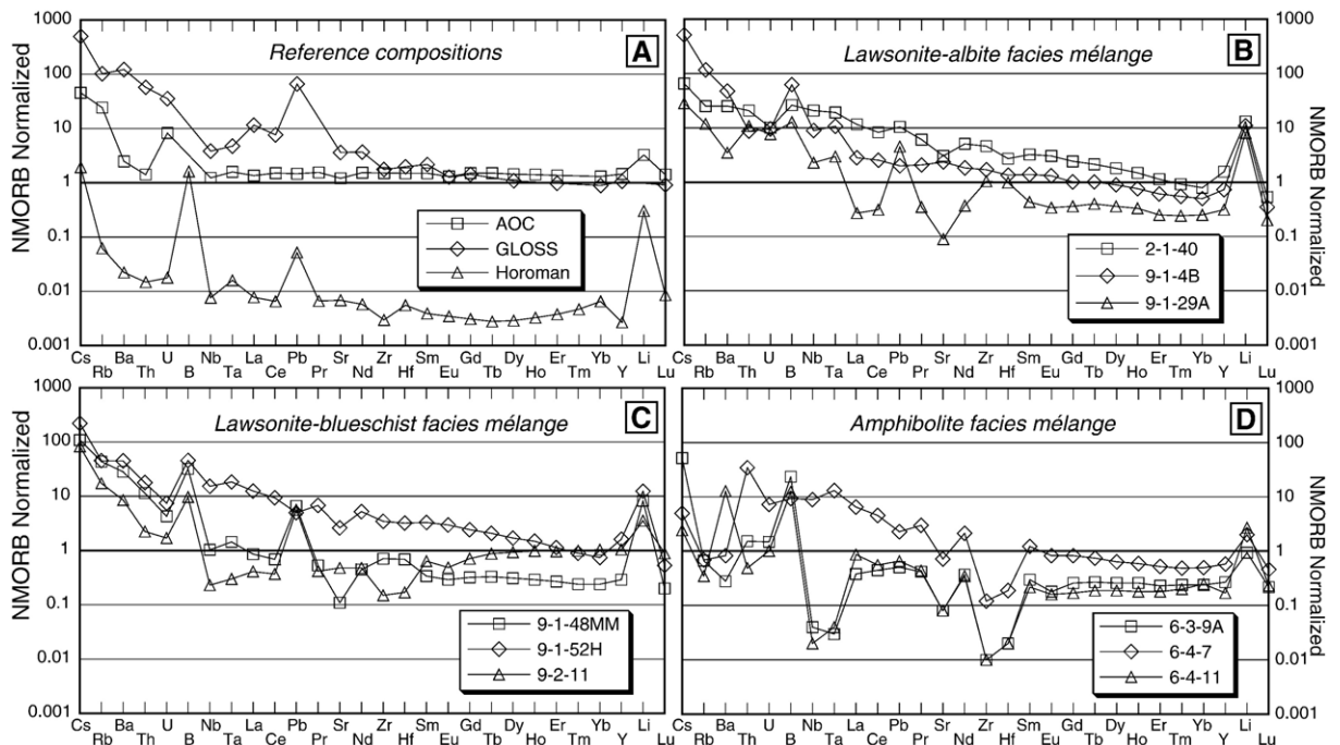
Fig. 6. NMORB-normalized [39] incompatible element diagrams for geochemical reference compositions (A) and mélangé matrix of the Catalina Schist (B–D). Reference compositions in A are the altered oceanic crust (AOC) composite of [3], estimated composition of global subducting sediment (GLOSS) of [2], and a depleted mantle composite composition (Horoman) based on the Horoman Peridotite complex of Japan [32,33] and depleted mantle data of [36]. Compositions for mélangé matrix were chosen to express typical incompatible element patterns and the full range in concentrations observed in each unit.
