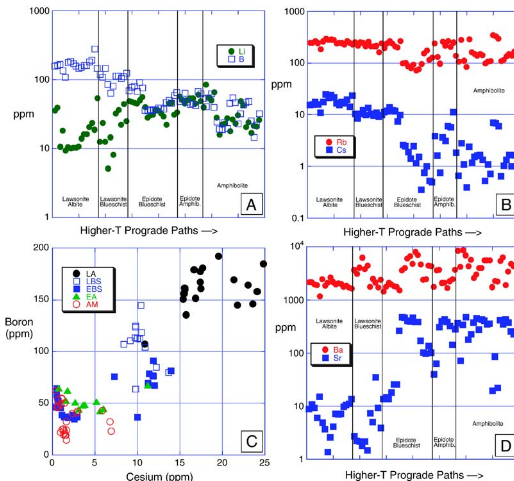
Fig. 4. Variations of concentrations of B, Li, Cs, Rb, Ba, and Sr in white micas in metasedimentary rocks (data for pegmatites and leucosomes, shown in Fig. 3, are not included) with increasing metamorphic grade (to the right). In these plots, the samples within each grade are ordered as in Fig. 3. (A) Plot of B and Li white-mica concentrations vs. grade, demonstrating the lower white-mica B concentrations, and higher white-mica Li concentrations, in rocks experiencing paths into metamorphic grades of epidote–blueschist and higher. (B) Plot of Rb and Cs white-mica concentrations vs. grade, demonstrating relatively uniform Rb concentrations across grades, and lower Cs concentrations in white micas in rocks experiencing paths into metamorphic grades of epidote–blueschist and higher. Note the greater increase in the Rb concentrations in the higher-grade units, presumably related to partitioning of some Rb into biotite at varying modal abundance. (C) Plot of Cs vs. B in white micas in the Catalina Schist metasedimentary rocks, demonstrating correlated decreases in concentration in higher-grade units. (D) Plot of Ba and Sr white-mica concentrations vs. grade, demonstrating relatively uniform Ba concentrations across grades, and higher Sr concentrations in white micas in rocks experiencing paths into metamorphic grades of epidote–blueschist and higher. Note the greater scatter in the Ba concentrations in the higher-grade units, presumably related to partitioning of some Ba into biotite at varying modal abundance. Note that these plots do not include data for fine-grained white mica believed to be retrograde in origin based on textures and mineral chemistry (see text for discussion).
