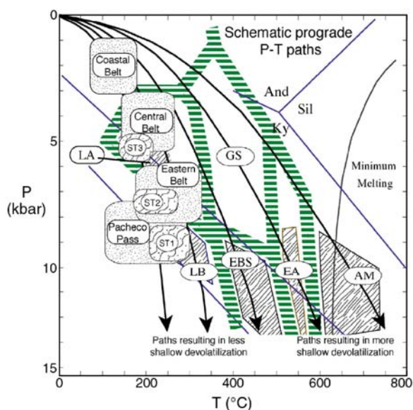
Fig. 1. Pressure–temperature diagram showing estimates of peak metamorphism for paleoaccretionary prism rocks from California, USA, and Mexico (see Grove and Bebout, 1995, for details regarding the generalized phase equilibria and stability fields compiled on this diagram). Arrows are schematic prograde P – T paths rocks might take in subduction zones, reflecting a wide range in thermal structure. LA = lawsonite–albite, LBS = lawsonite–blueschist, EBS = epidote–blueschist, GS = greenschist, EA = epidote–amphibolite, and AM = amphibolite. Various units of the Coast Ranges Franciscan Complex are indicated (“Coastal Belt”, “Central Belt”, and “Eastern Belt”, in order of increasing peak metamorphic pressures thus depths of underthrusting; see Sadofsky and Bebout, 2003, 2004; Blake et al., 1987). Also indicated is the peak P – T for the Franciscan Complex metagreywackes at Pacheco Pass, California (estimates from Ernst, 1993). Fields labeled “ST1”, “ST2”, and “ST3” indicate peak conditions for tectonometamorphic units of the Western Baja Terrane (from Sedlock, 1988).
