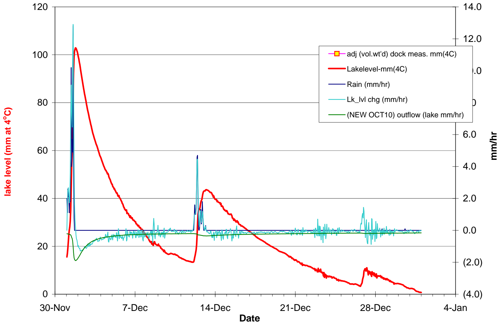
L. Lacawac Hourly avg Lake level, Lake level change/hr, Rain/hr Free flow w/o beavers in Nov; lake ice cover starting 9Dec10 (complete damping of waves 16Dec10)
