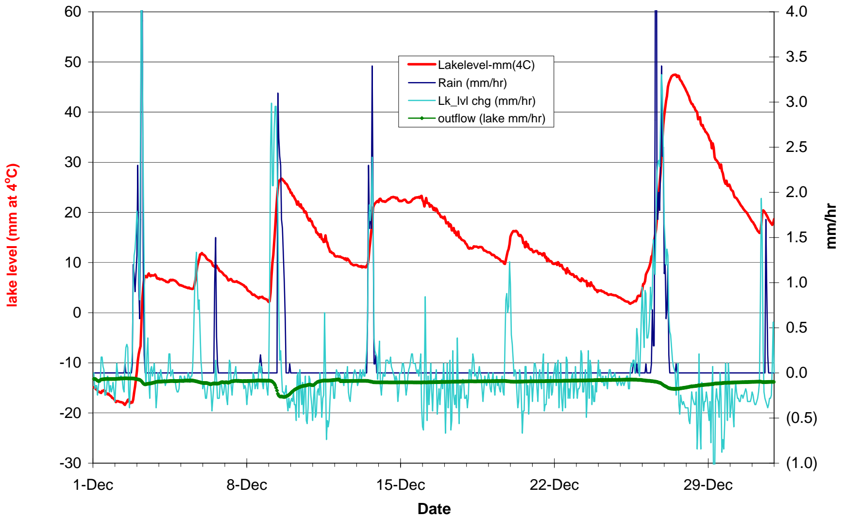
L. Lacawac Hourly avg Lake level, Lake level change/hr, Rain/hr snow 5-6Dec (5"), 9Dec, 19Dec, 31Dec (melt in gage = delayed "rain"); Tw indicates ice cover 12-15Dec, full on 18Dec
