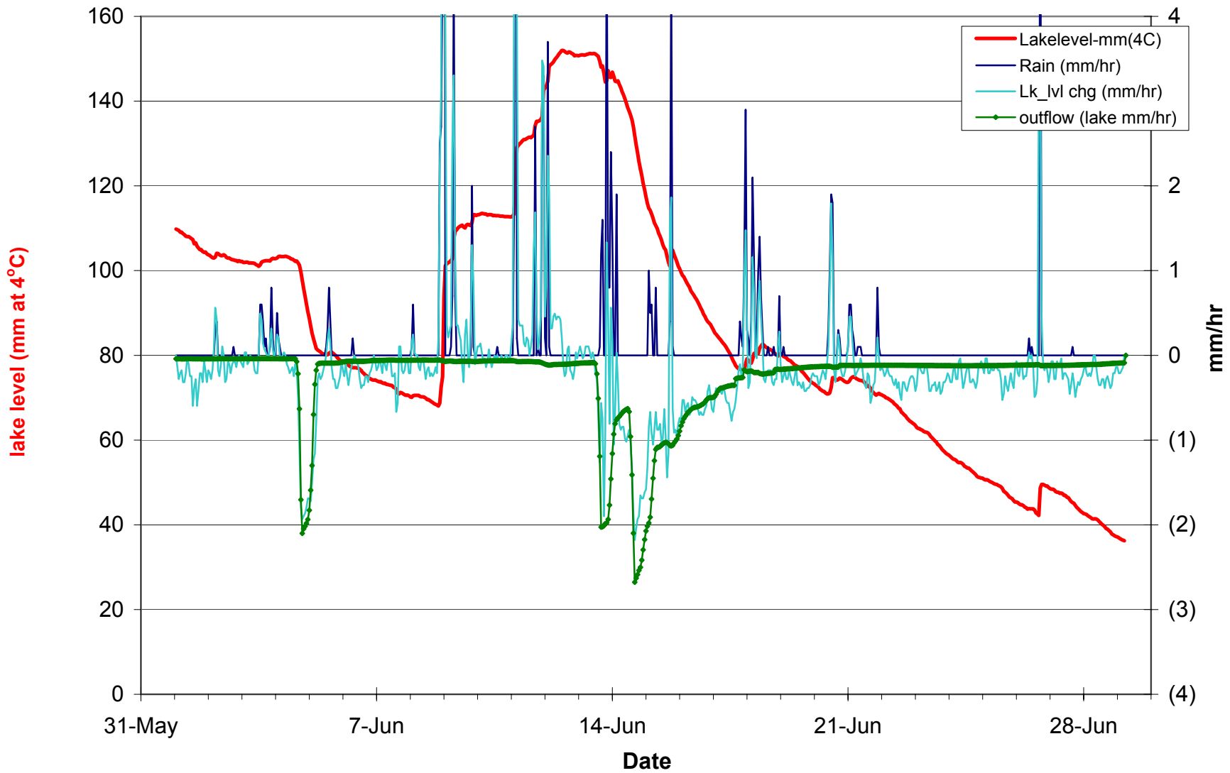
Hourly avg Lake level, Lake level change/hr, Rain/hr Stn moved to dock & beaver dam leaking observed 9Nov08; dam breakup on 4,13,14Jun; outflow models revised in Jun09 for beaver dam height & outflow logger data
