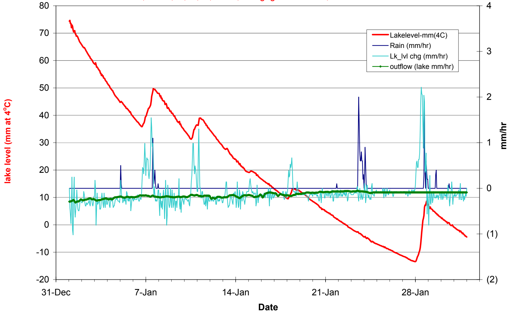
Hourly avg Lake level, Lake level change/hr, Rain/hr Stn moved to dock & beaver dam leaking observed 9Nov08; outflow modeled from lake level; snow 6-7, 10-11,13,15,18,28Jan; rain gage melt 23-24, rain28Jan
