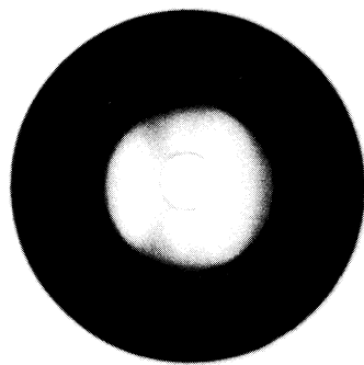
Fig. 2. Photomicrograph showing the contact area (innermost circle) resulting from the contact between a lens ( R = 0.72 mm) and a flat sheet of \text{PDMS}^{\text{ox}}\text{-O}_3\text{Si}(\text{CH}_2)_{10}\text{CH}_3 under zero load. The radius of contact deformation was \sim 92 \mu\text{m} .
